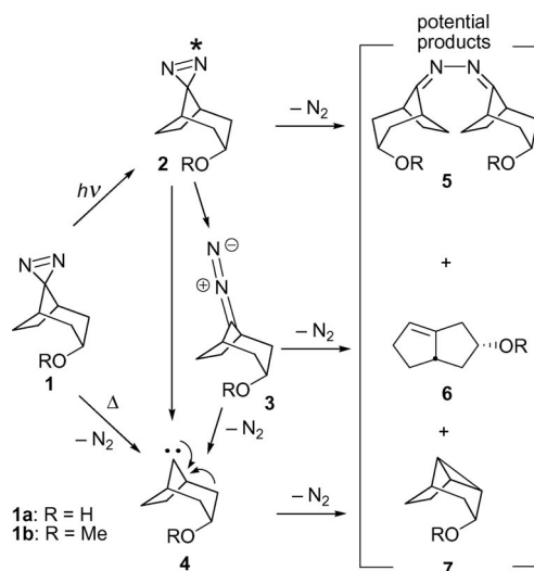
Scheme 1. Potential reactions of diazirines 1 .
