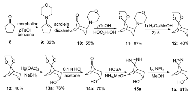
Scheme 2. Synthesis of carbene precursor 1a .
