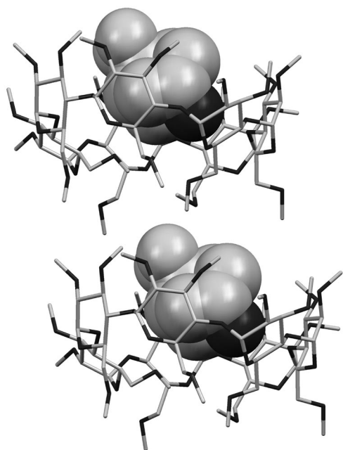
Figure 1. Crystal structure of 1a@TRIMEB showing the packing of the complex. [17b] The hydrogen atoms are omitted for clarity.
