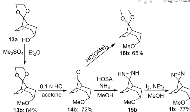
Scheme 3. Synthesis of carbene precursor 1b .
